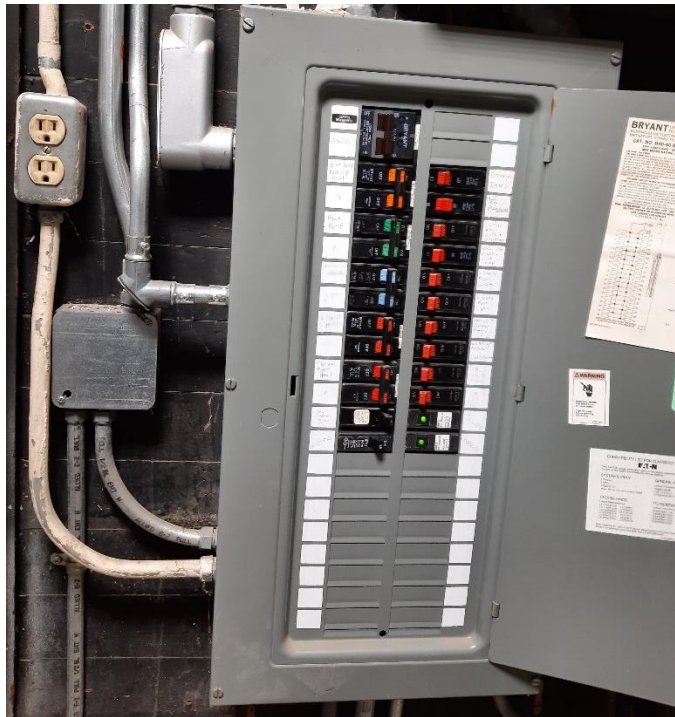
Inside of Electrical Panel – City of Naches side
