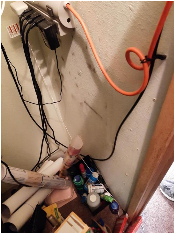
Inside of Network Closet with Location of Dedicated Circuit – Naches Library side
